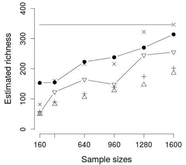
Figure 6. Richness average estimation by size. The thick gray line is the real richness. The black circles are the AQS estimations, the triangles are the CHAO estimations and the inverted triangles are the ACE estimations. The symbols x and + are the extrapolation ACE estimation and the bound extrapolation ACE estimation respectively.
