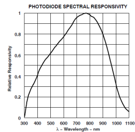
Figura 4 – TSL12T, TSL13T LIGHT-TO-VOLTAGE CONVERTERS
